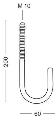
5020-A Tirante zincato Zinc-plated tie-rod
