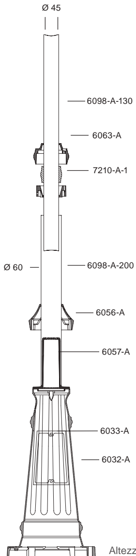
Palo telescopico 60/45 - Telescopic pole 60/45
